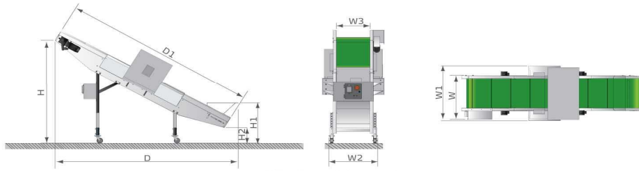
PNL-MS Outline Drawings
