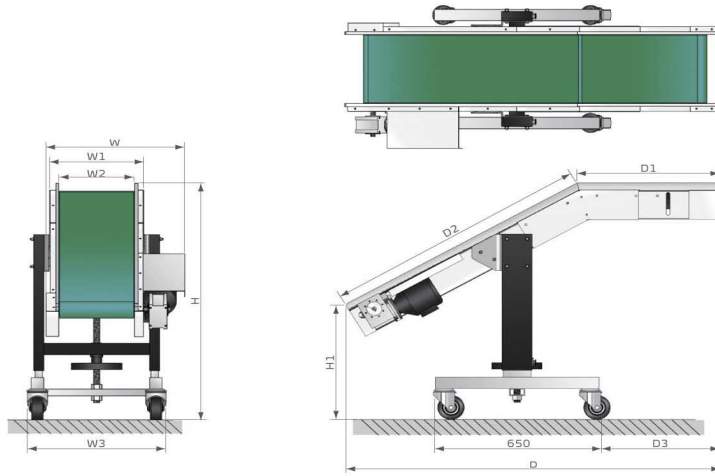
SV Outline Drawings
