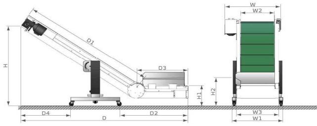
CB Outline Drawing
