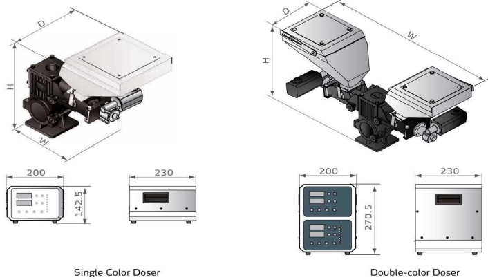
Single Color Doser
